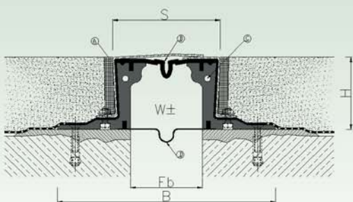
500/NcL-070
